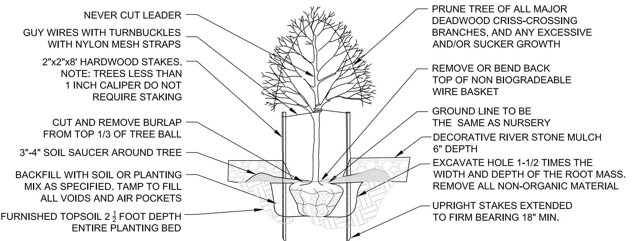
TREE PLANTING – BALLED AND BURLAPPED NOT TO SCALE
