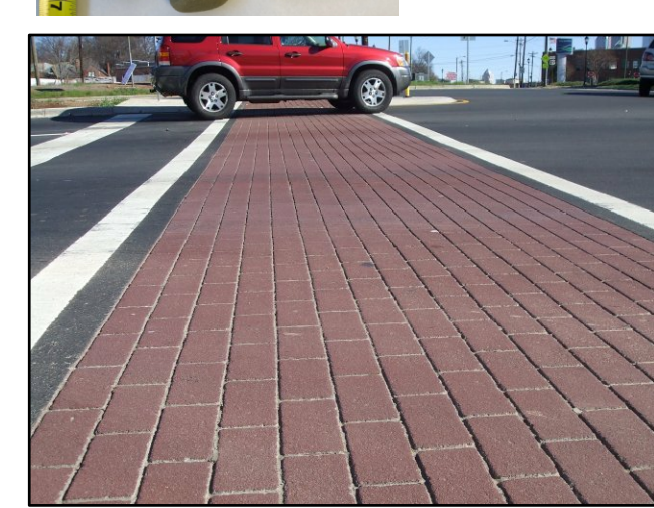
STAMPED ASPHALT BRICK – RUNNING BOND
