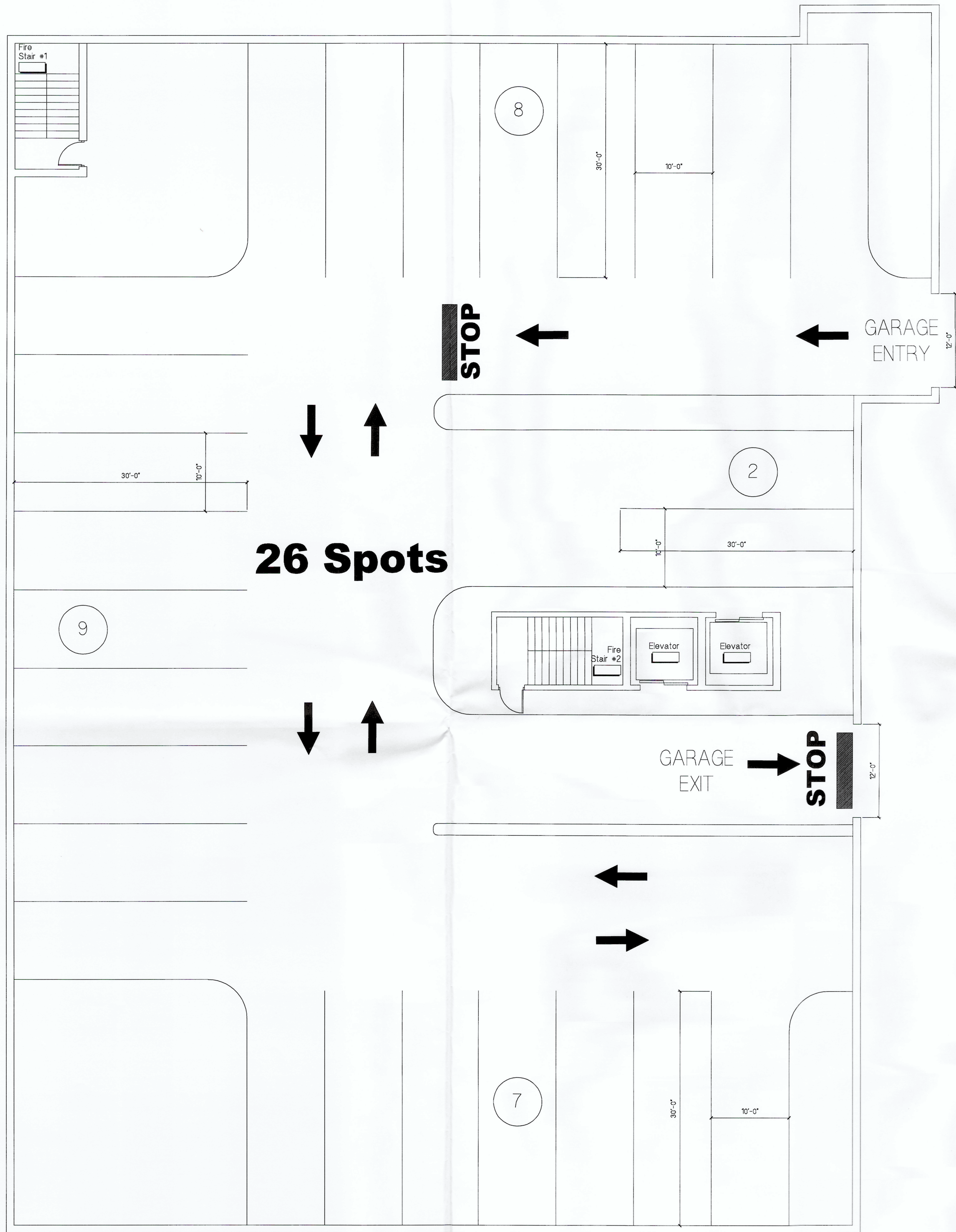
1 Lower Level Construction Plan A-100 SCALE: 1/8"=1'-0"
